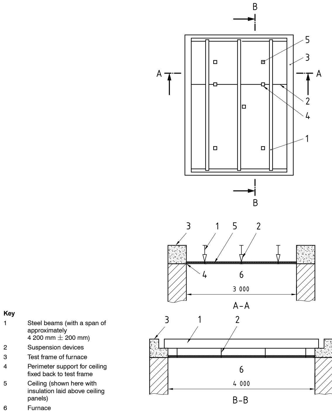
Figure 1 — Ceiling exposed to fire from below — Suspended (shown) or self-supporting
