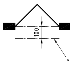
Figure A.3 — Regular pyramid — Example of measurement of gas temperature and pressure
