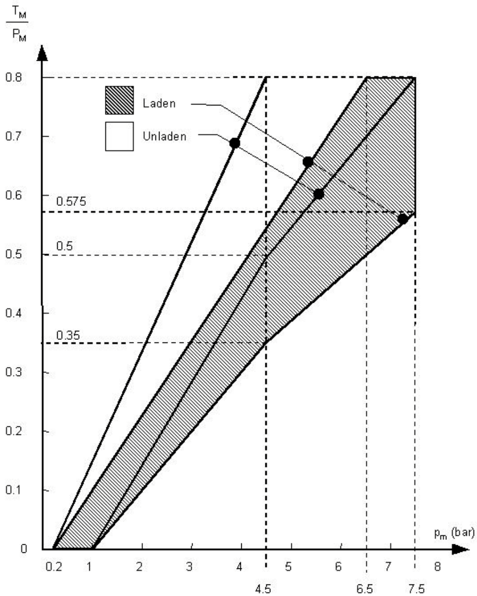
DIAGRAM 3 TRACTORS FOR SEMI-TRAILERS (see paragraph 3.1.6. of this annex)
