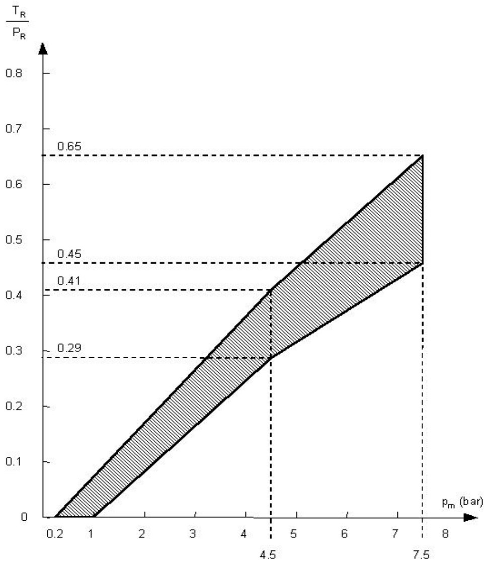
DIAGRAM 4A SEMI-TRAILERS (see paragraph 4. of this annex)
