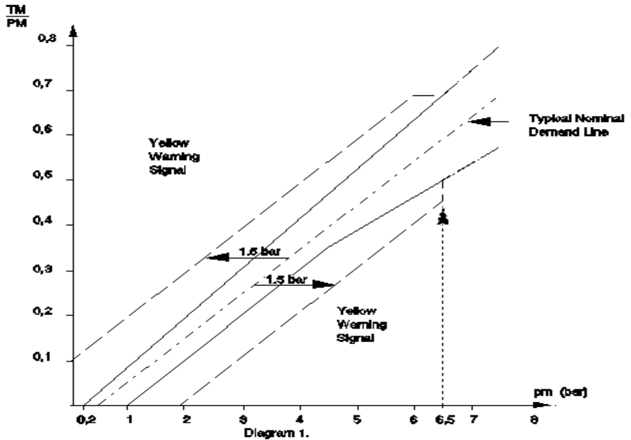
Towing Vehicles for Trailers (except semi-trailers)
