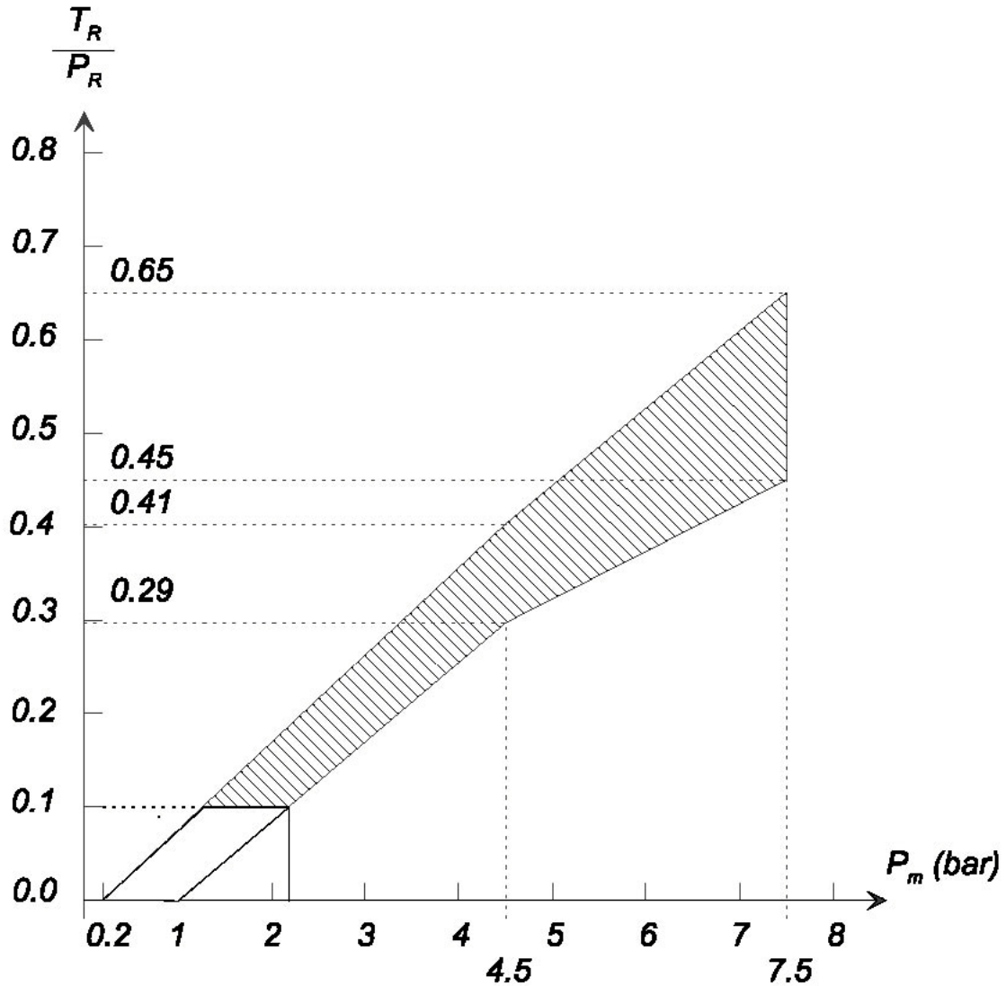
DIAGRAM 4A SEMI-TRAILERS (see paragraph 4. of this annex)
