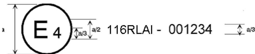
Figure 6 (see paragraph 4.4.3.7. of this Regulation)
