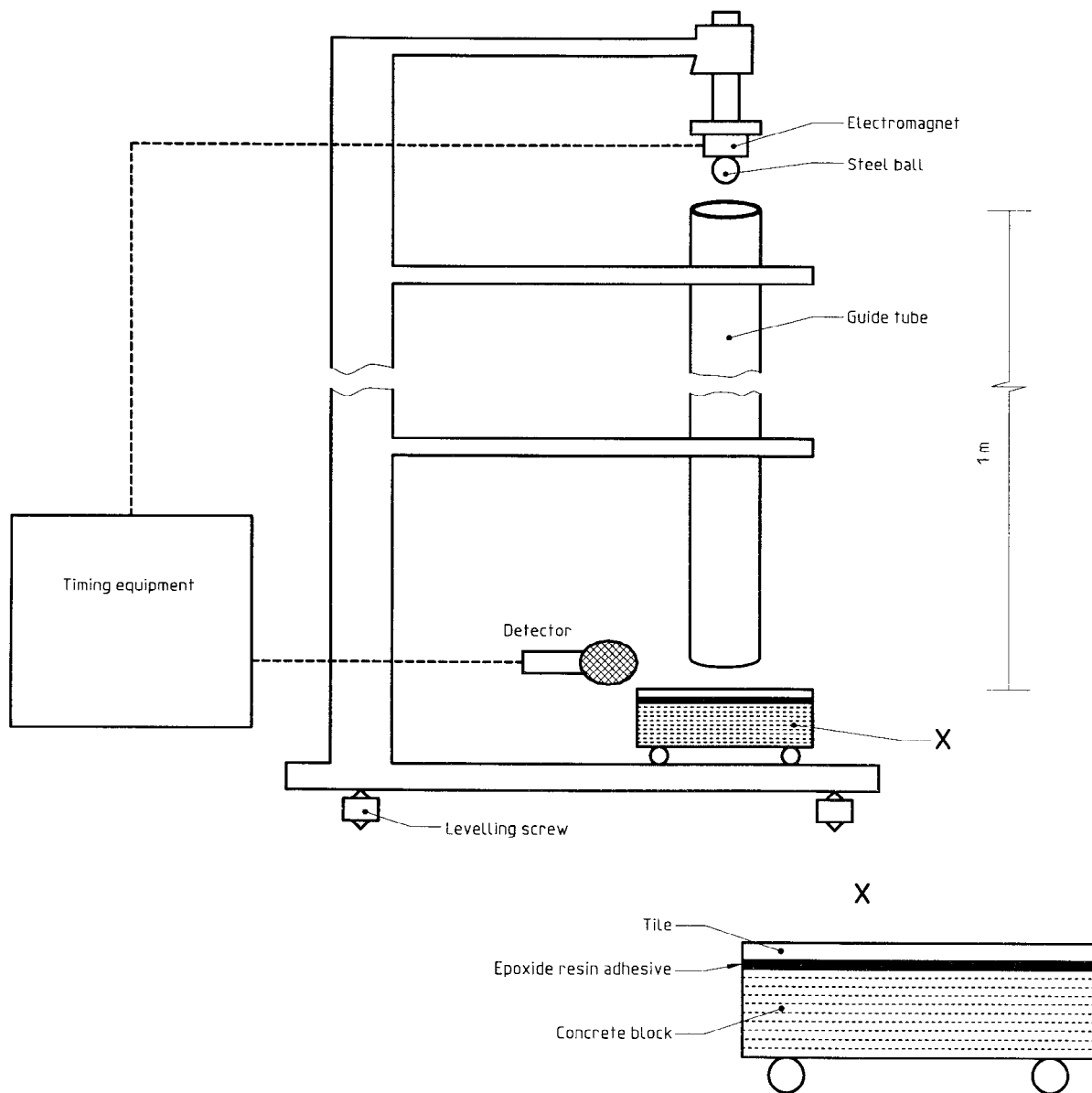
Figure 1 — Ball-release apparatus
