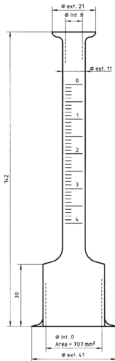
Figure A.1 — Apparatus for measuring the surface water absorption of concrete blocks or slabs
