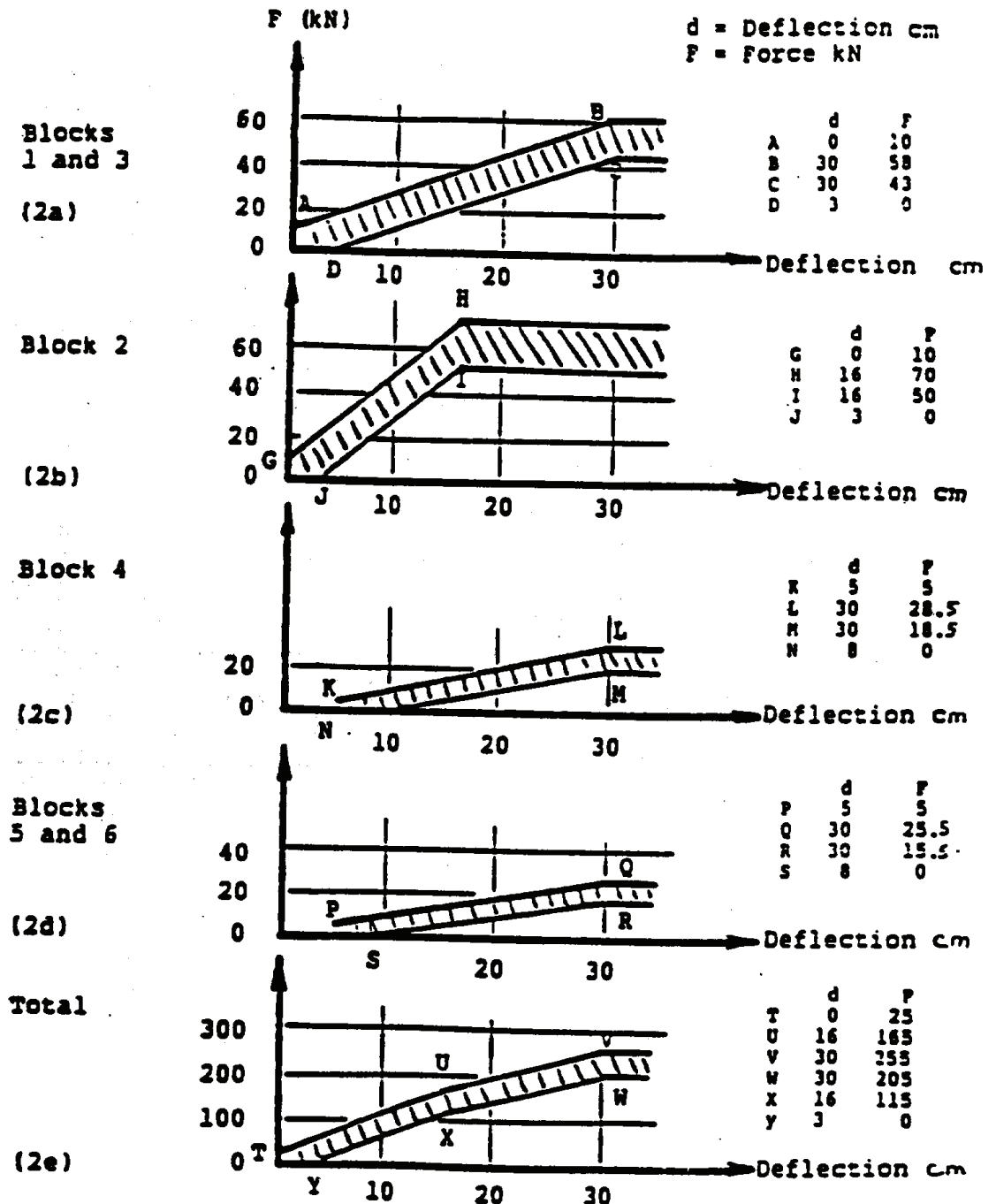
Figure 2 Force-deflection curves
