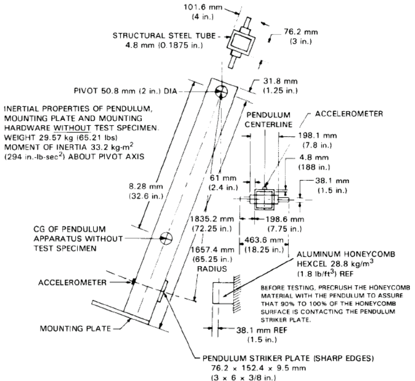
Figure 5 - Neck pendulum specification according to American Code of Federal Regulation (49 CFR Chapter V Part 572.33)
