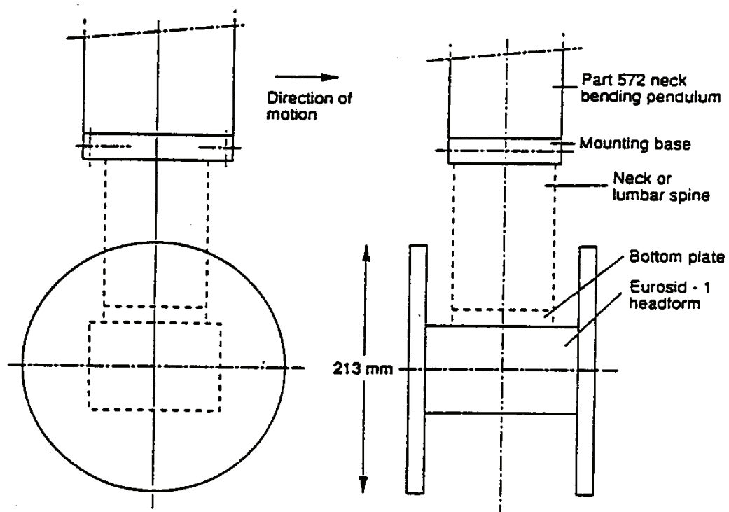
Figure 4 - NECK AND LUMBAR SPINE CERTIFICATION TEST SET-UP
