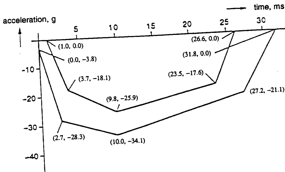
Figure 6 -PENDULUM DECELERATION-TIME CORRIDOR FOR LUMBAR SPINE CERTIFICATION TEST
