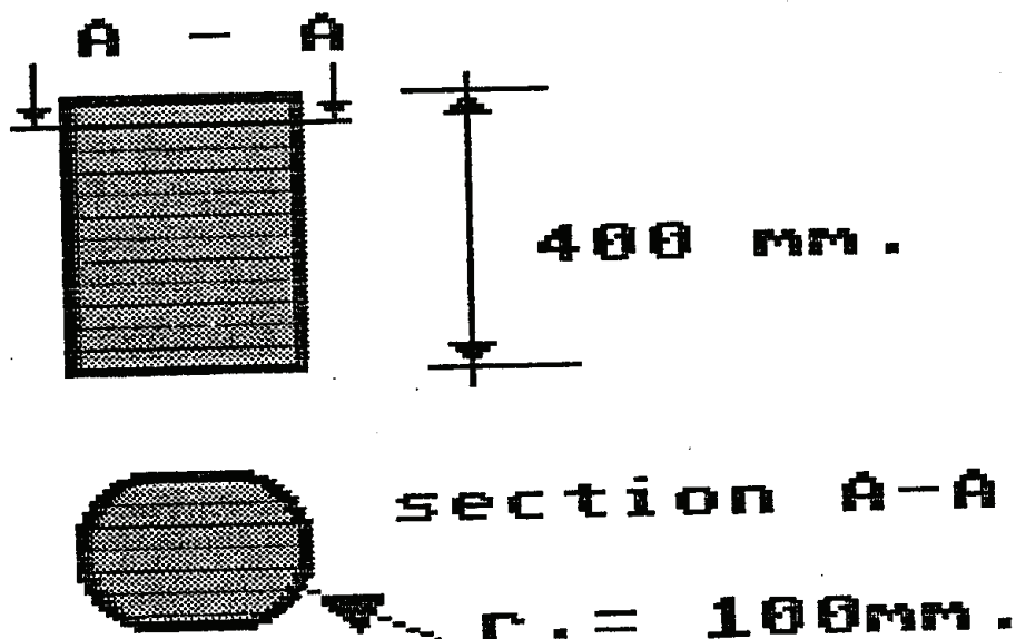
FIG. 2 head form impactor
