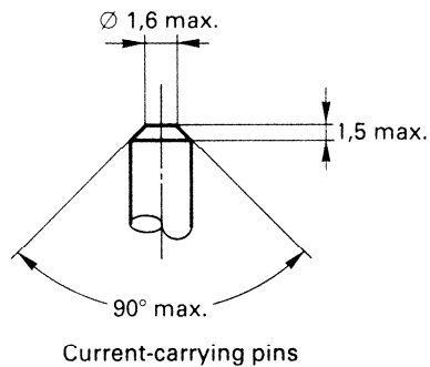
Current-carrying pins
