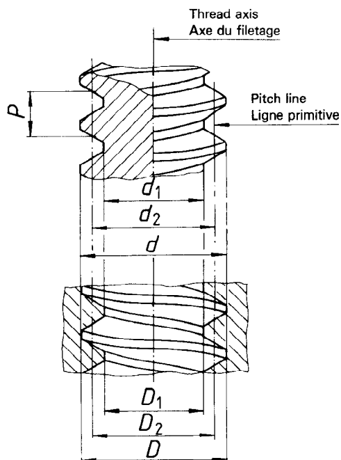
Figure 10 — Diameter symbols for internal and external threads
