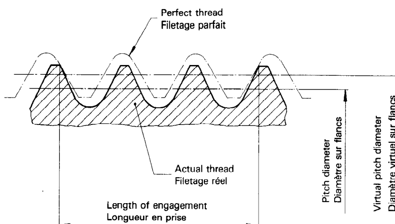
Figure 12 — Virtual pitch diameter of an actual thread
