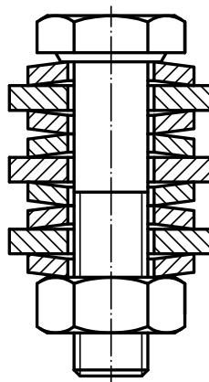
Figure 4 — Test apparatus for conical spring washers
