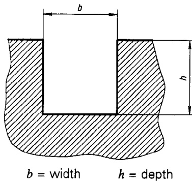
Figure 4 — "N"-type notch
