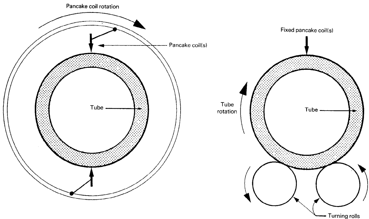
Figure 1 — Simplified diagram of concentric coil technique
